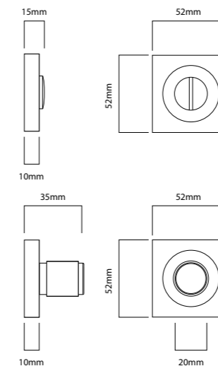
BERLIN SQUARE PRIVACY TURN
