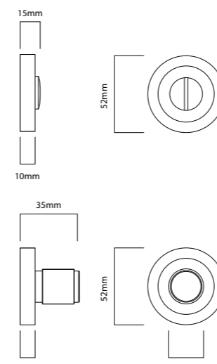
BERLIN ROUND PRIVACY TURN
