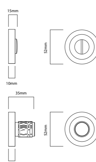
BRUNSWICK ROUND PRIVACY TURN
