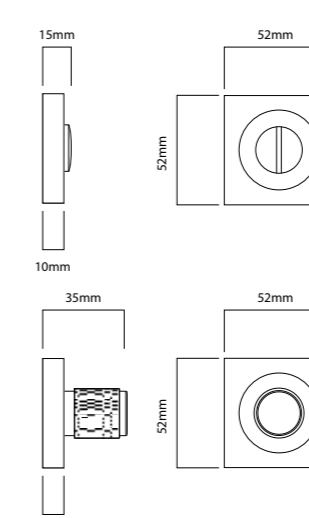
BRUNSWICK SQUARE PRIVACY TURN
