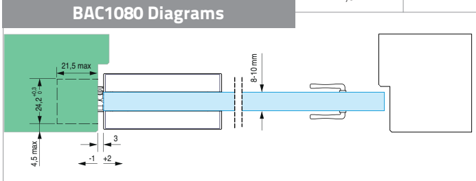
Hinge rebated 4.5mm max from edge of jamb on opening side
