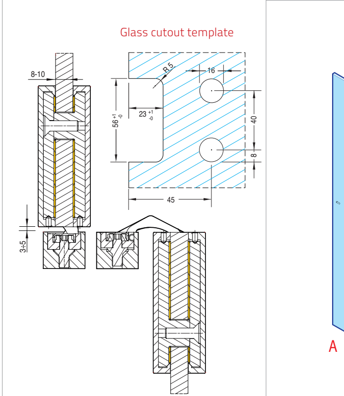
Hinge rebated 4.5mm max from edge of jamb on opening side
