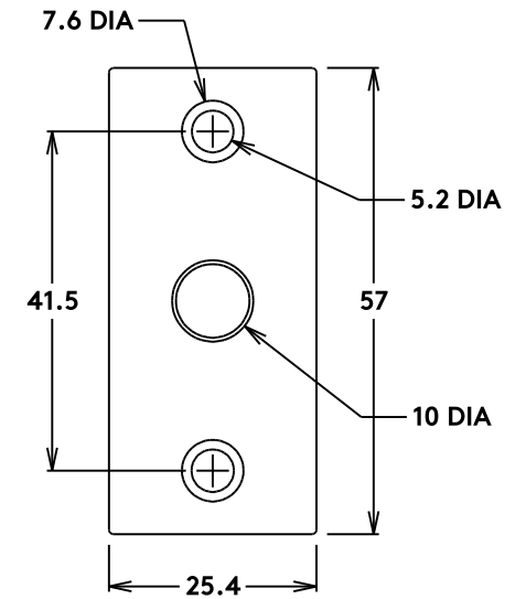
Faceplate
