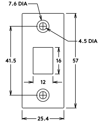
Faceplate
