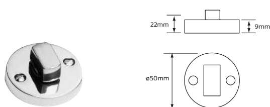
Turn #27
