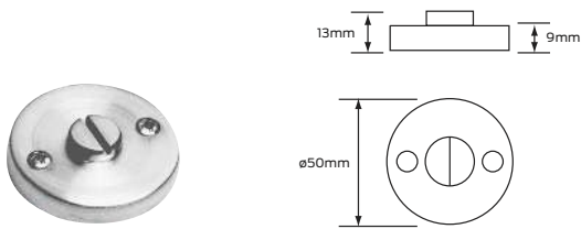
Emergency release #24
