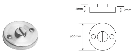
Emergency release #28
