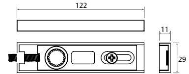
Top Pivot Housing
