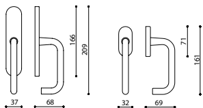
C125R - fixed window slider
