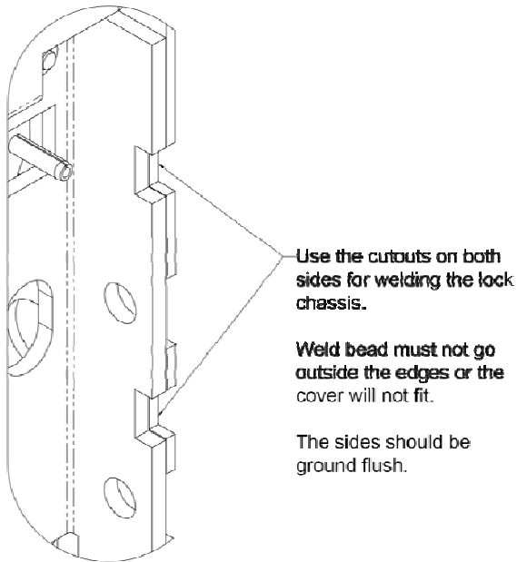
Figure 4. Chassis Welding
