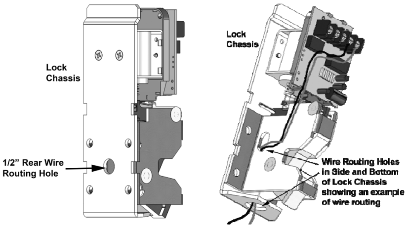
Figure 7. Wire Routing
