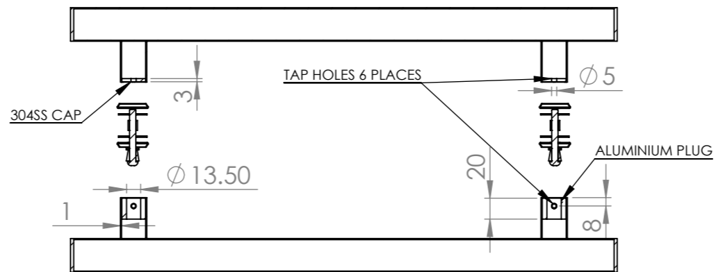
SECTION C-C
