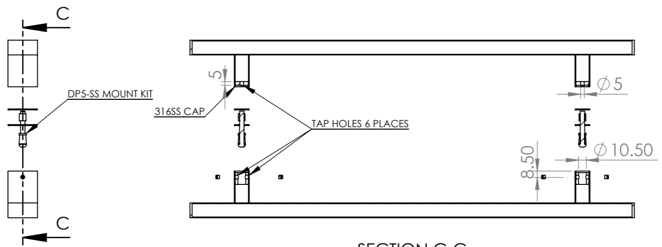
SECTION C-C
