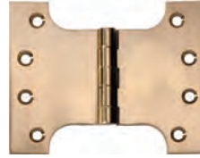
2481 PB (W125xH100xT4mm)
